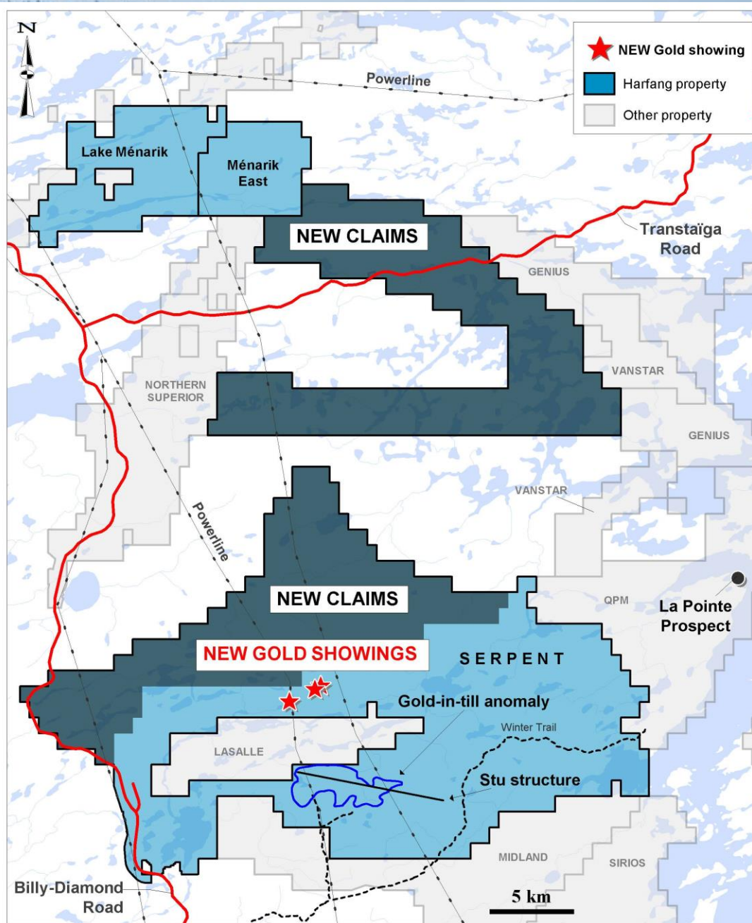
Figure 1. Location of the Serpent Property (James Bay, Québec) and the new claims shown in dark blue. The new gold showings discovered during fall 2020 exploration campaign are located on the map.
